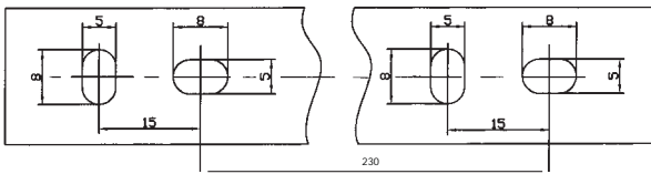
20mm width cable trunking
