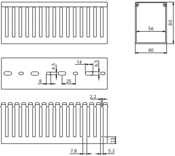
60x80 slotted trunking
