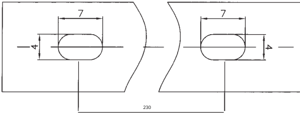
16mm width cable trunking
