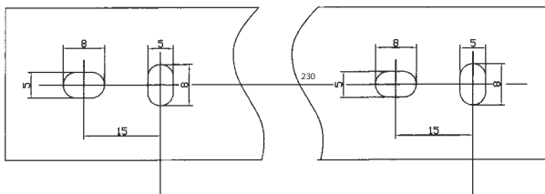
40mm width cable trunking
