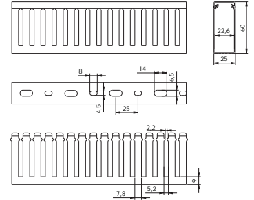
25x60 slotted trunking
