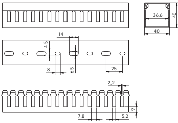
40x40 slotted trunking
