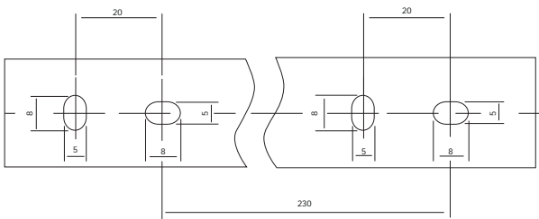
25mm width cable trunking
