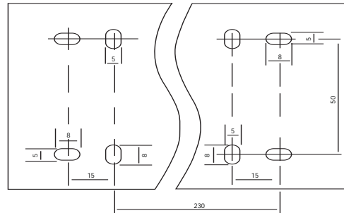
110mm width cable trunking
