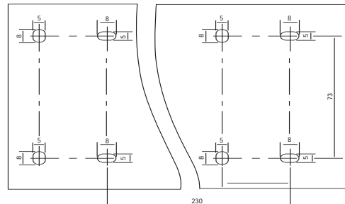
120mm width cable trunking
