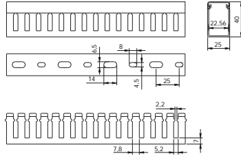
25x40 slotted trunking
