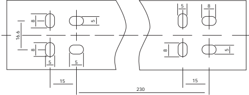
60mm width cable trunking
