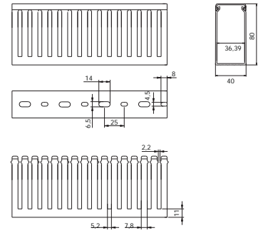
40x80 slotted trunking
