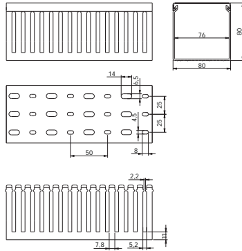
80x80 slotted trunking
