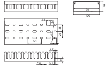
100x40 slotted trunking
