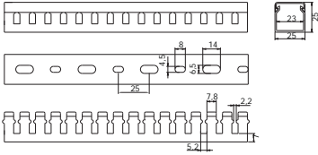
25x25 slotted trunking
