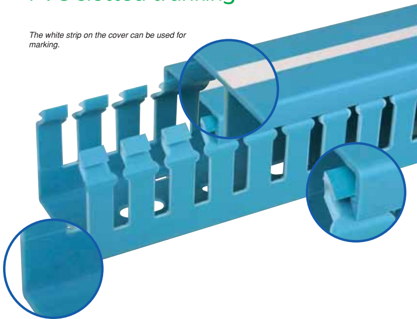
PKS Line slotted trunking
