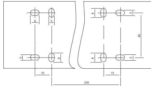
100mm width cable trunking
